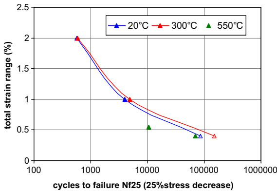
Fig. 3. Low cycle fatigue test results for Eurofer 97 HIP joints. Open symbols stand for interrupted tests (no failure).
