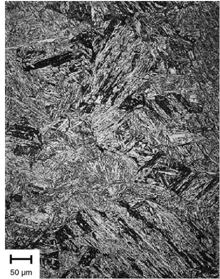
Fig. 8. Microstructure of the weld zone, Eurofer TIG weld.
