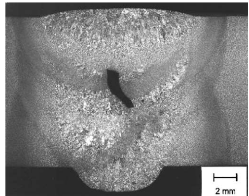
Fig. 9. Intentional lack of fusion defect in 14 mm thick Eurofer weld (macrography).
