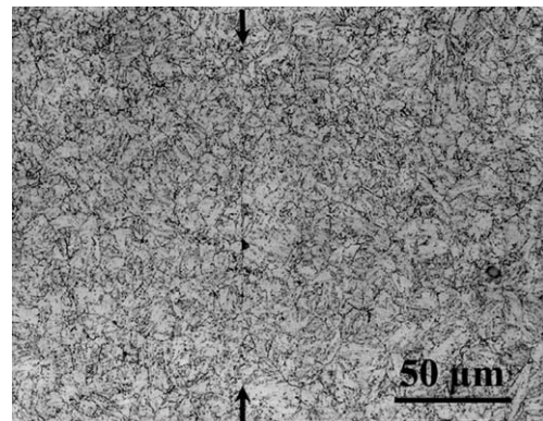
Fig. 1. Microstructure of a Eurofer 97 1100 °C HIP joint.
